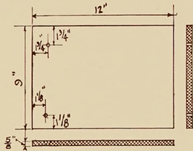
PLAN AND SECTION OF SHINGLE TILE
