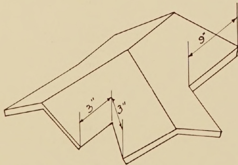
SKETCH OF FINIAL
