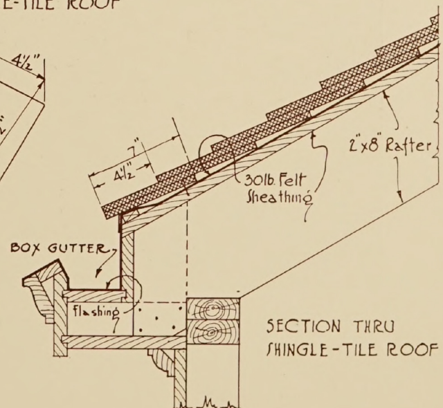
SKETCH OF SHINGLE-TILE ROOF
