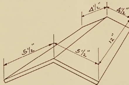
SKETCH OF HIP TILE
