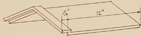
SKETCH OF RIDGE TILE
